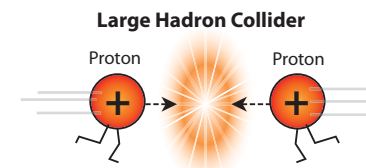
The Large Hadron Collider at CERN in Europe collides protons with protons, making it harder to pick out the asymmetries. But it can reach higher energies than those used at the Tevatron.
