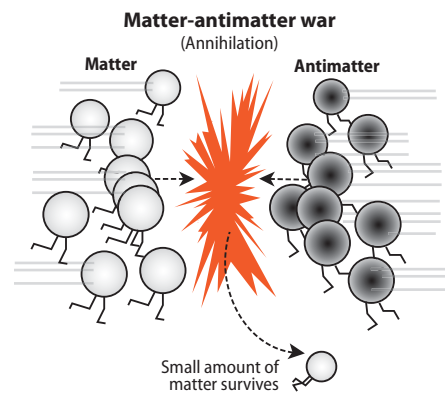
Antimatter and matter should have annihilated each other in a flash of radiation. Yet somehow, a small amount of matter survived this encounter. Why? All illustrations: Astronomy: Roen Kelly
