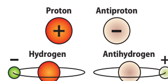
Both hydrogen and antihydrogen atoms have the same physical characteristics, like chemical reactions and spectra. So, scientists can’t differentiate hydrogen from antihydrogen in distant objects.
