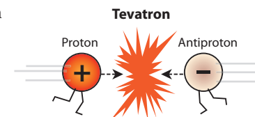
The Tevatron at Fermilab outside Chicago slams together protons and antiprotons, making it easy to pick out the asymmetry of the collision products.
