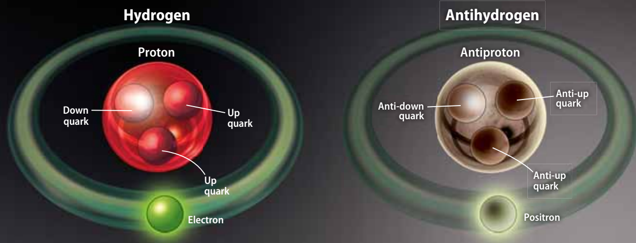
A hydrogen atom is made up of an electron and a proton (two “up quarks” and one “down quark”). An antihydrogen atom is exactly opposite — it holds a positron and an antiproton (two anti-up quarks and one anti-down quark). Astronomy: Roen Kelly
